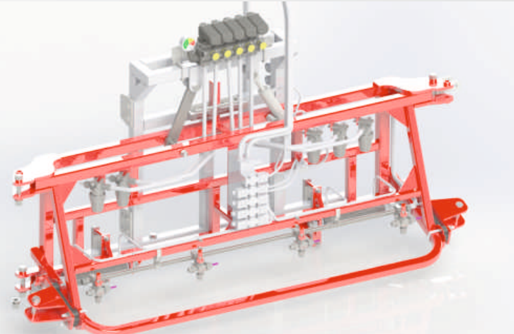
Hydraulic cylinder for tilting in option.
